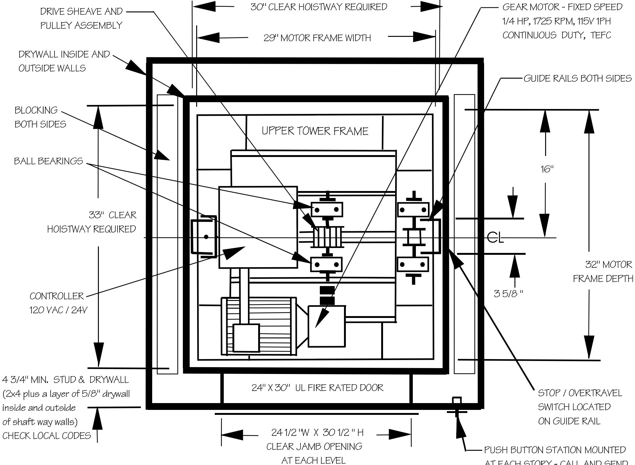
BUTLERS BUDDY COMMERCIAL LIFT 24 W X 30 DP X 30 HIGH
