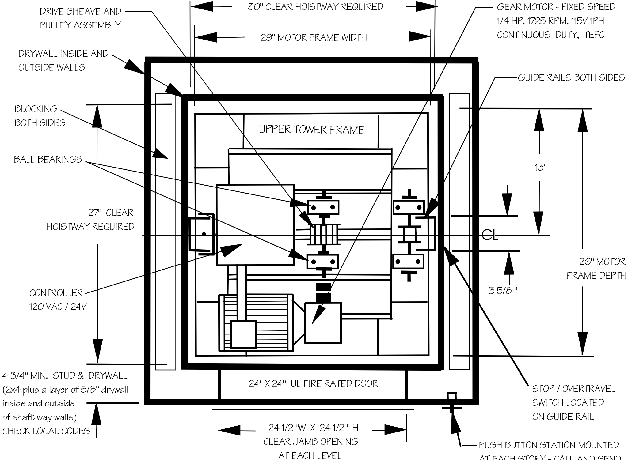
BUTLERS BUDDY COMMERCIAL LIFT 24 W X 24 DP X 24 HIGH
