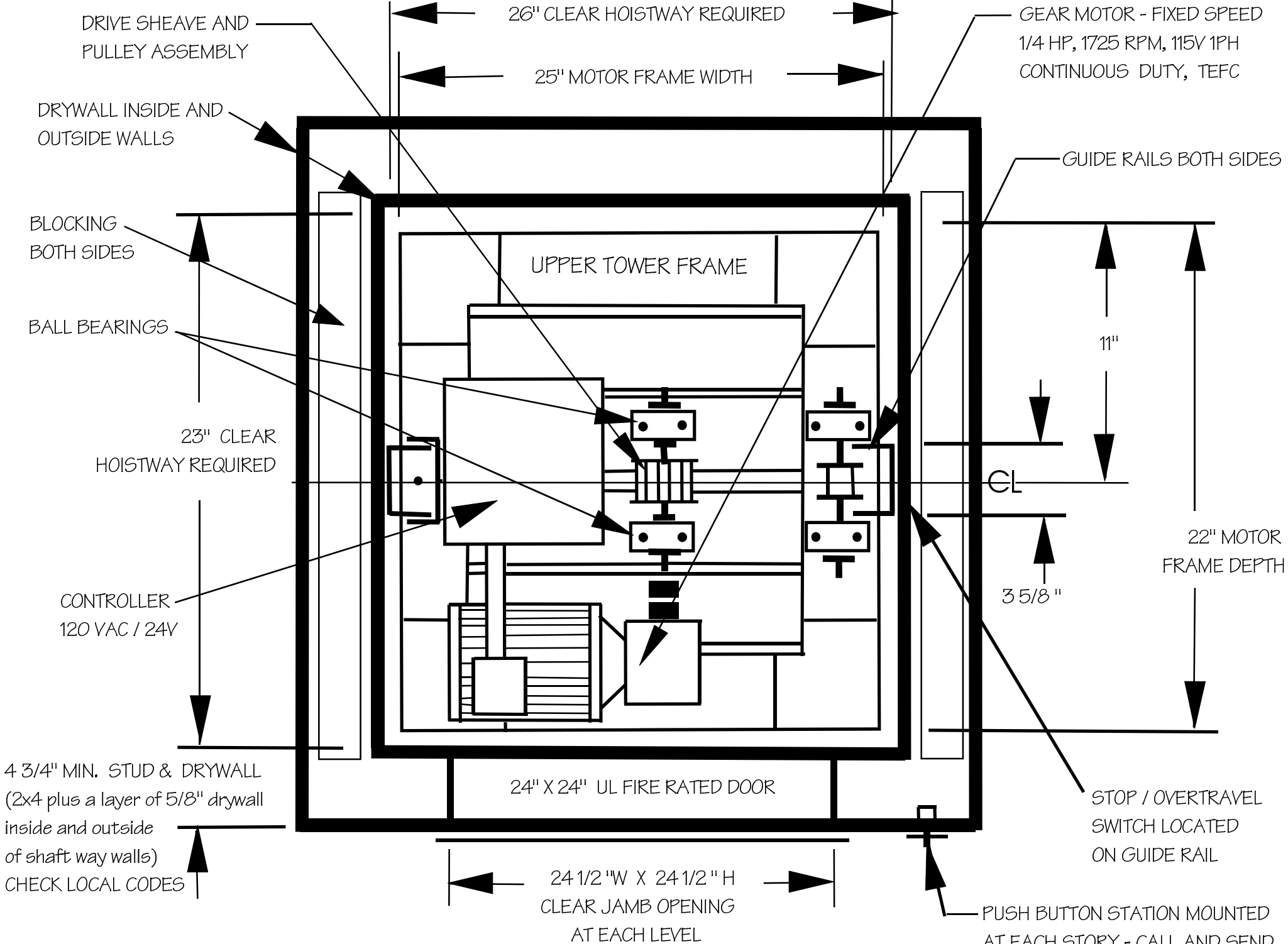
BUTLERS BUDDY COMMERCIAL LIFT 20 W X 20 DP X 24 HIGH
