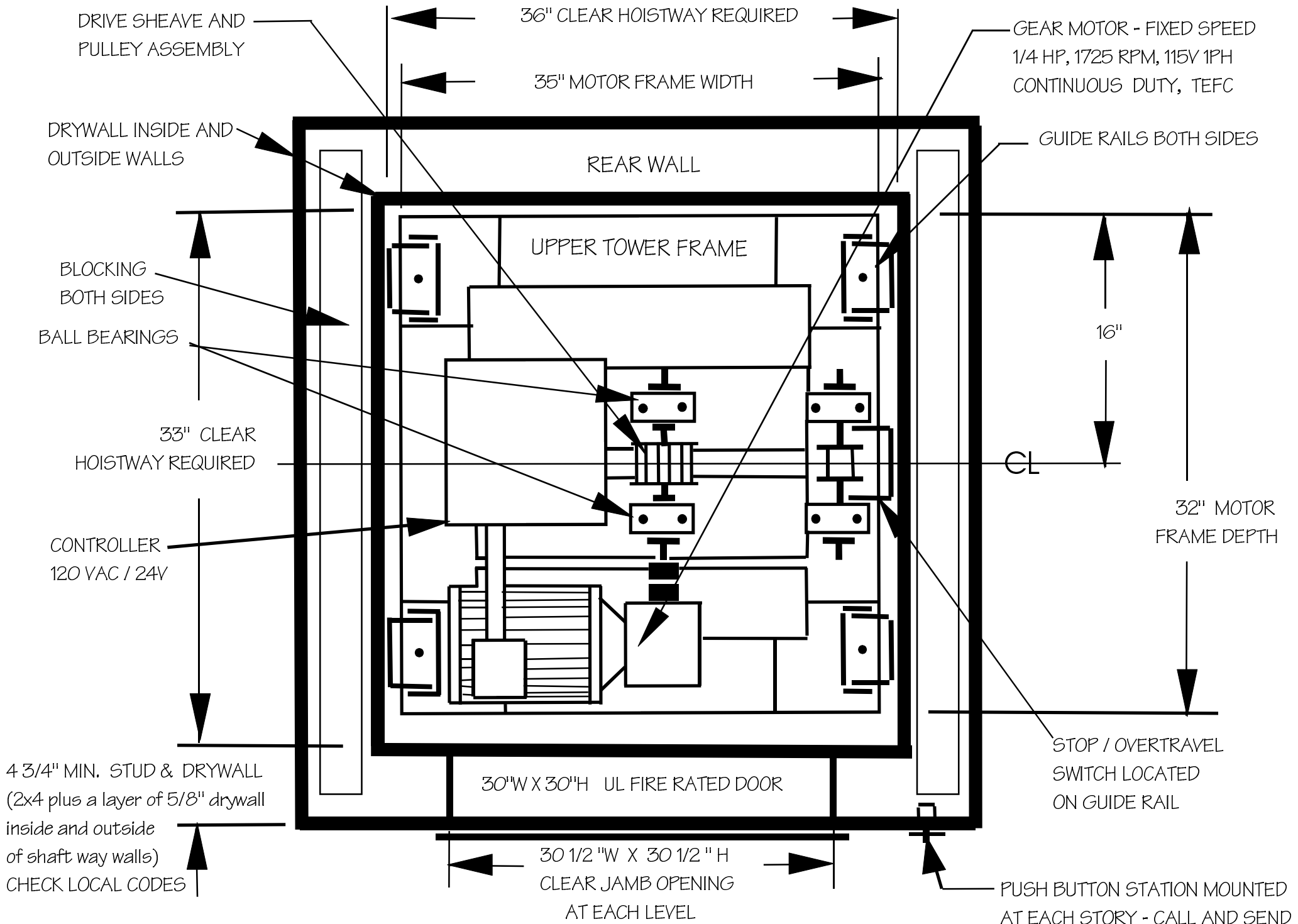
DOUBLE GUIDE / SINGLE BELT DUMBWAITER 30" W X 30" DP X 30" HIGH
